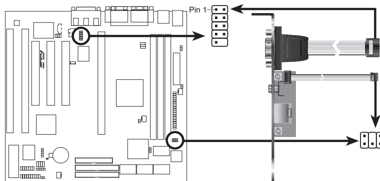
P2L-VM/P2E-VM Serial COM 2 + TV-Out Bracket
